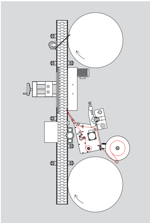
Above sketch indicates a lay-out with feeding and collection tables
